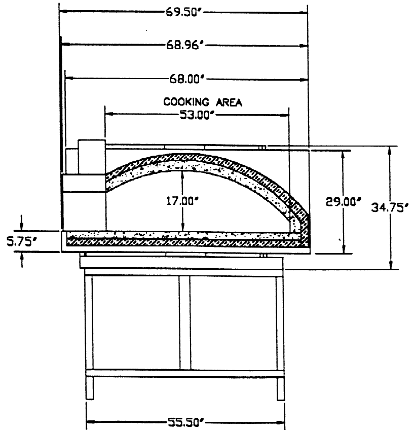
CUT-OFF VIEW
