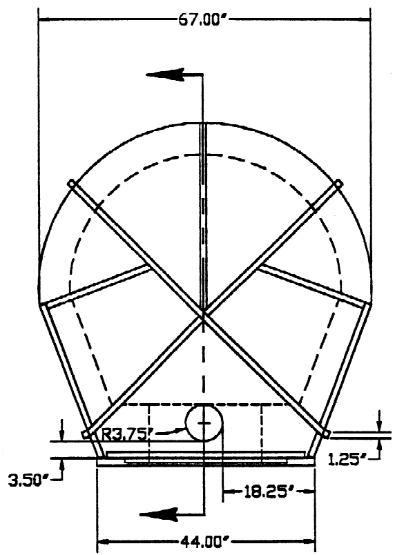
TOP VIEW
