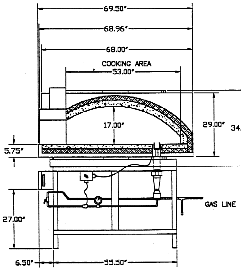
CUT-OFF VIEW
