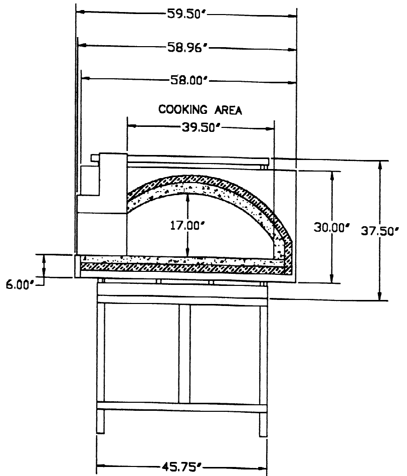
CUT-OFF VIEW
