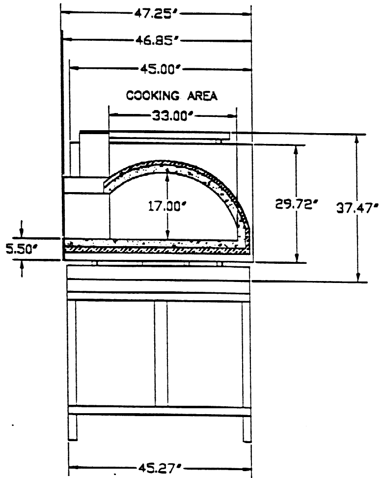
CUT-OFF VIEW
