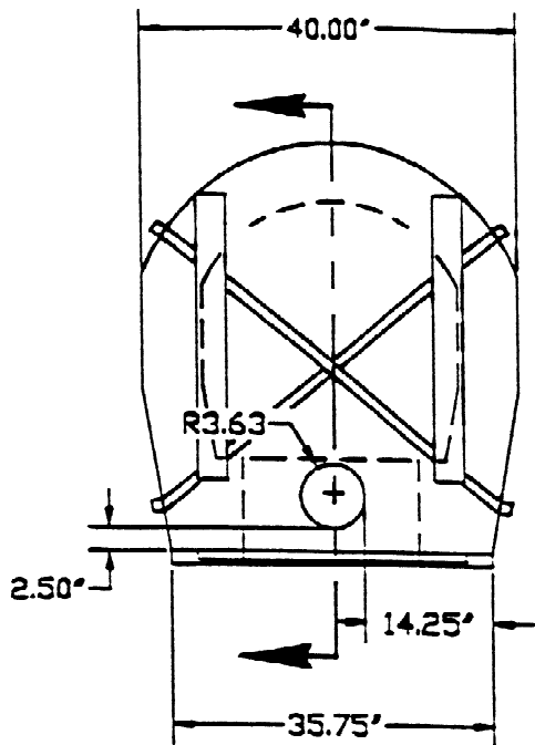
TOP VIEW
